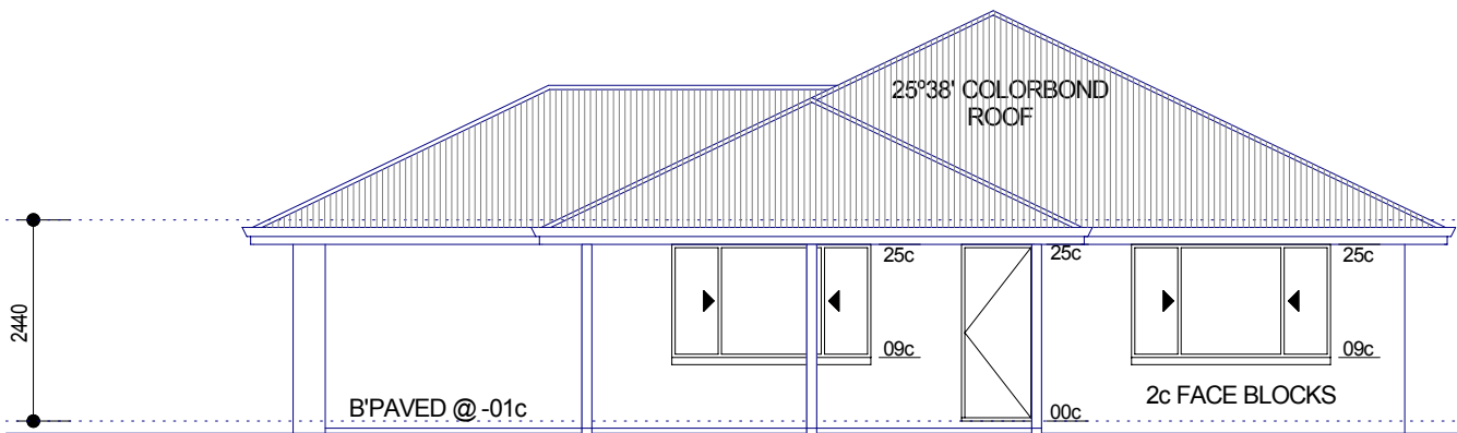
Front Elevation 1:100
